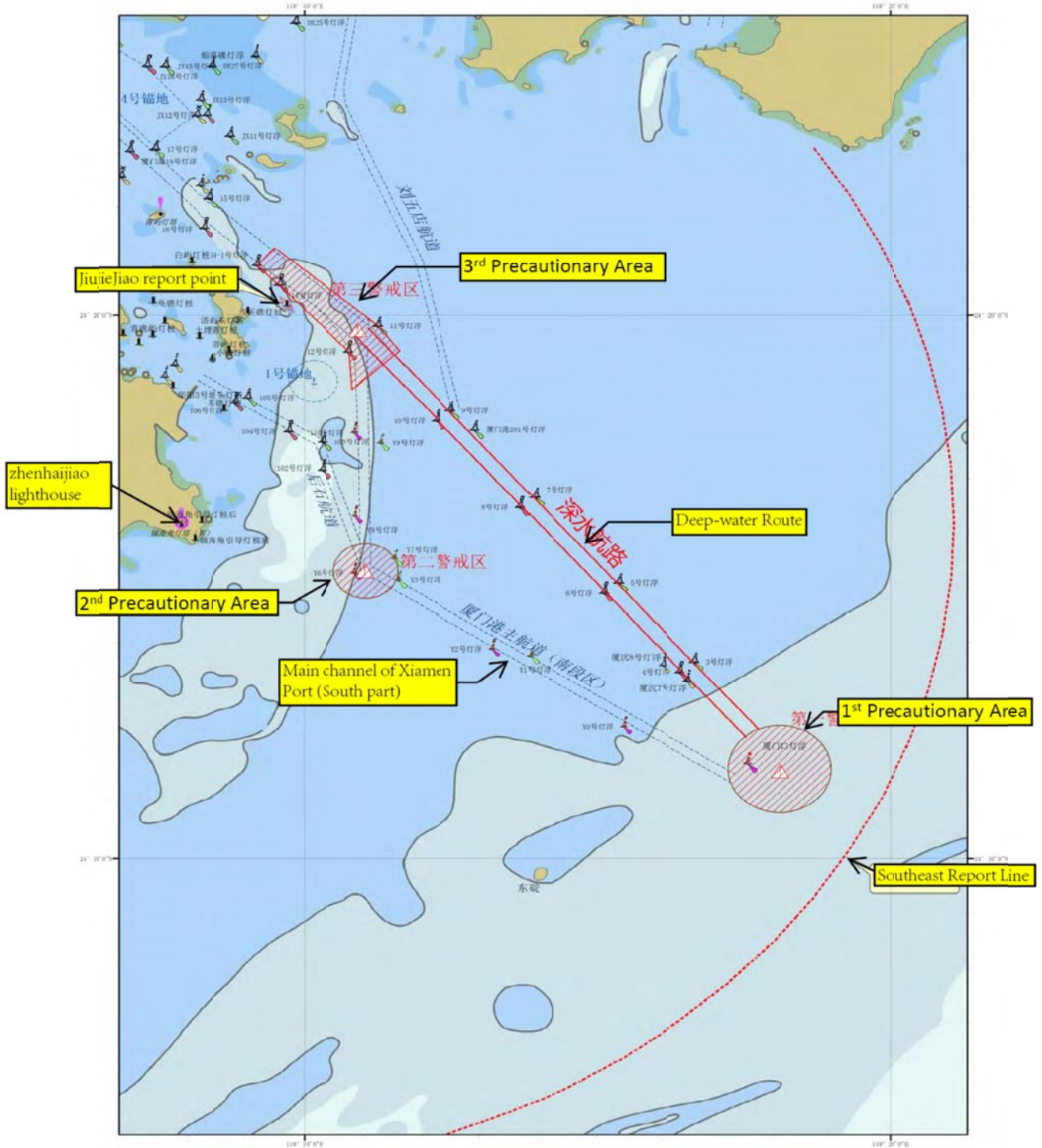
Sketch II of Ship Routing System in Xiamen Water Area
